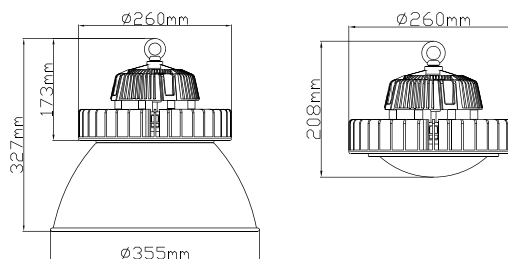
Dimension of 60° alum reflector
