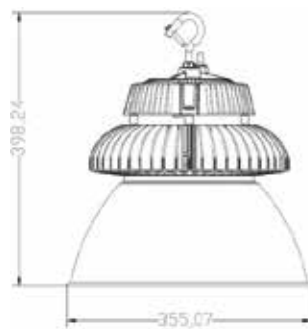
Dimension of 60° alum reflector
